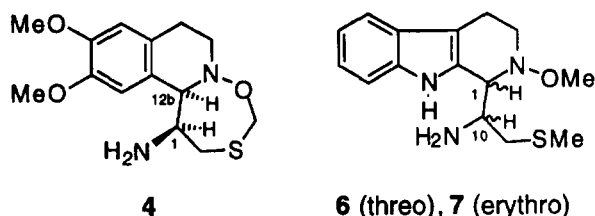
Chart 1. Naturally tetracyclic eudistomin derivatives together with the discussed synthetically derived analogues.
