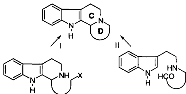
Scheme 1. Synthetic strategies towards tetracyclic \beta -carboline.
