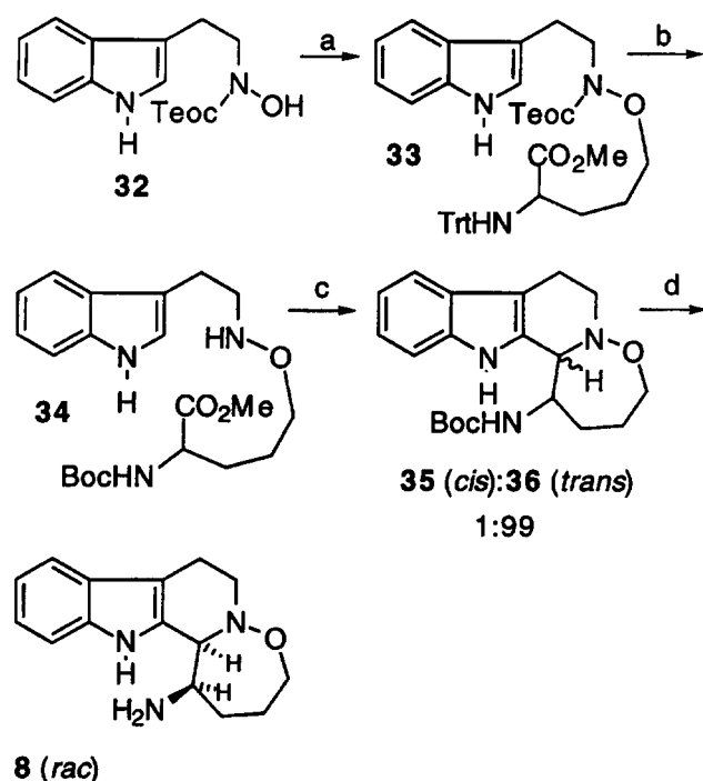
Scheme 7. Synthesis of the eudistomin desulfo carba derivative 8 . Reagents: (a) (i) NaH, DME, (ii) 31 ; (b) (i) 0.1 N HCl, F_3CCH_2OH , (ii) (BOC)_2O , Et_3N , CH_2Cl_2 , (iii) KF \cdot 2H_2O , n-Bu_4NCl , MeCN; (c) (i) DIBAL, CH_2Cl_2 , -75^\circ C , (ii) TFA; (d) TMSI, MeCN ( 35 only).
