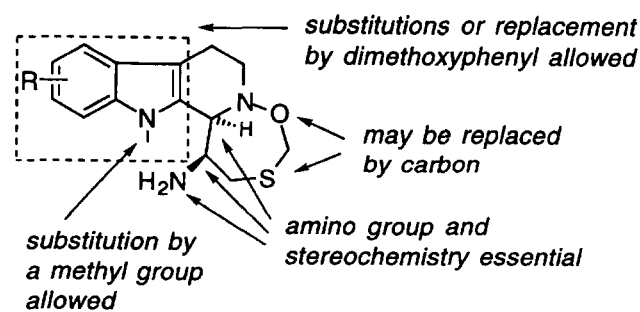
Chart 3. Schematic representation of the SAR conclusions.
