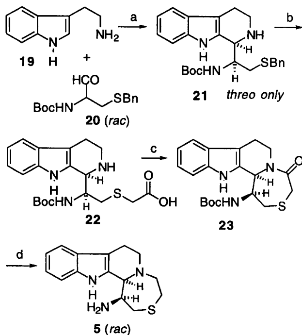
Scheme 4. Synthesis of the eudistomin deoxo carba derivative 5 . Reagents: (a) TFA, \text{CH}_2\text{Cl}_2 ; (b) (i) Na, \text{NH}_3(\text{l}) , (ii) methyl chloroacetate, DBU, benzene, (iii) 2 N NaOH, dioxane; (c) TBTU, DiPEA, DMF; (d) TMSI, MeCN.
