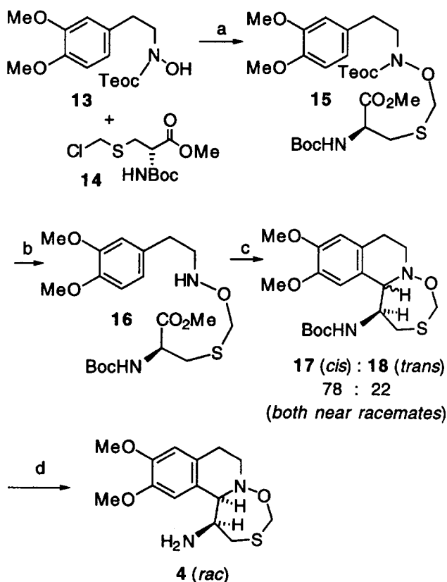
Scheme 3. Synthesis of the eudistomin isoquinoline derivative 4 . Reagents: (a) NaH, NaI, DME; (b) \text{KF}_2\cdot\text{H}_2\text{O} , n\text{-Bu}_4\text{NCl} , MeCN, 50^\circ\text{C} ; (c) i. DIBAL, \text{CH}_2\text{Cl}_2 , -75^\circ\text{C} , ii. TFA, -75^\circ\text{C} –rt; (d) TMSI, MeCN ( 17 only).
