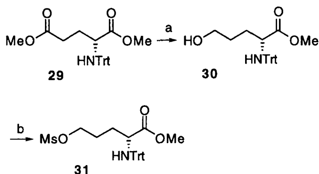
Scheme 6. Selective functionalization of the \delta -carboxyl group of glutamic acid by shielding of the \alpha -carboxylate with the bulky N -trityl protective group. Reagents: (a) \text{LiAlH}_4 , \text{Et}_2\text{O} , 0 °C; (b) \text{MsCl} , \text{Et}_3\text{N} , \text{Et}_2\text{O} , -20 °C.
