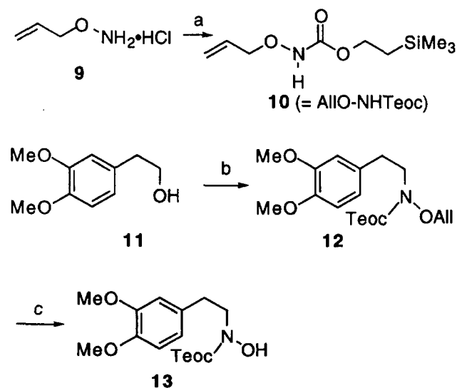
Scheme 2. Application of the Mitsunobu reaction for the synthesis of \beta -phenyl-N-hydroxy ethylamines. Reagents: (a) 2-(trimethylsilyl)ethoxycarbonyl chloride, DiPEA, THF; (b) 10, DIAD, PPh 3 , THF; (c) Pd(OAc) 2 , PPh 3 , Et 3 N·HO 2 CH, MeCN:H 2 O (4:1), reflux.
