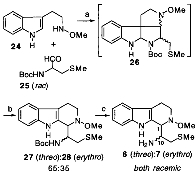
Scheme 5. Synthesis of the D-ring-opened eudistomin derivatives 6 and 7 . Reagents: (a) TFA, \text{CH}_2\text{Cl}_2 ; (b) two days; (c) TMSI, MeCN.
